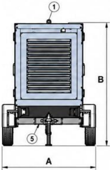
VISTA FRONTAL
